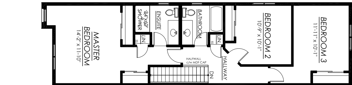
2ND FLOOR PLAN
