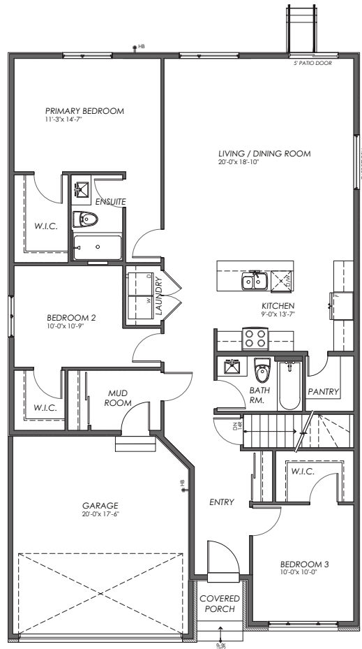
MAIN FLOOR
